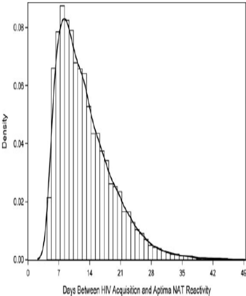
Figure 1. Simulated eclipse period probability density function (PDF) translated from a 3-parameter Weibull prior distribution. Parameters for location, shape, and
